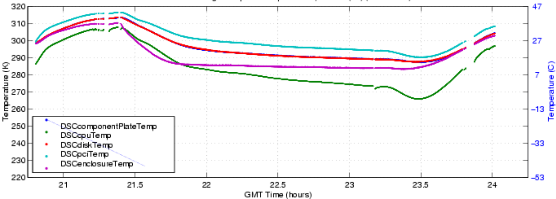
S-HIS Data Storage Computer Temperatures , 041015 (fbf) (ENG Plot 8)
