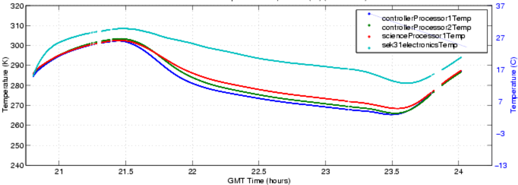
S-HIS Electronics Temperatures 1/2, 04-10-15 (fbf) (ENG Plot 7)
