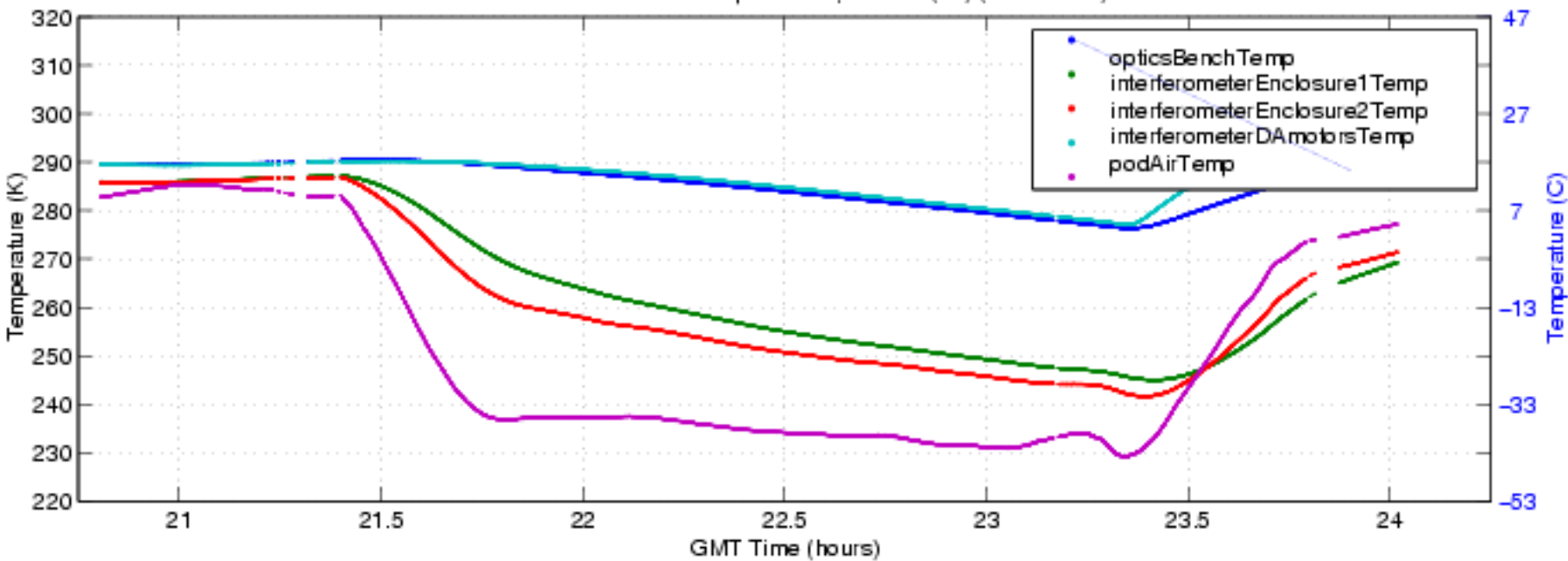
S-HIS Interferometer Temperatures, 041015 (bf) (ENG Plot 5)
