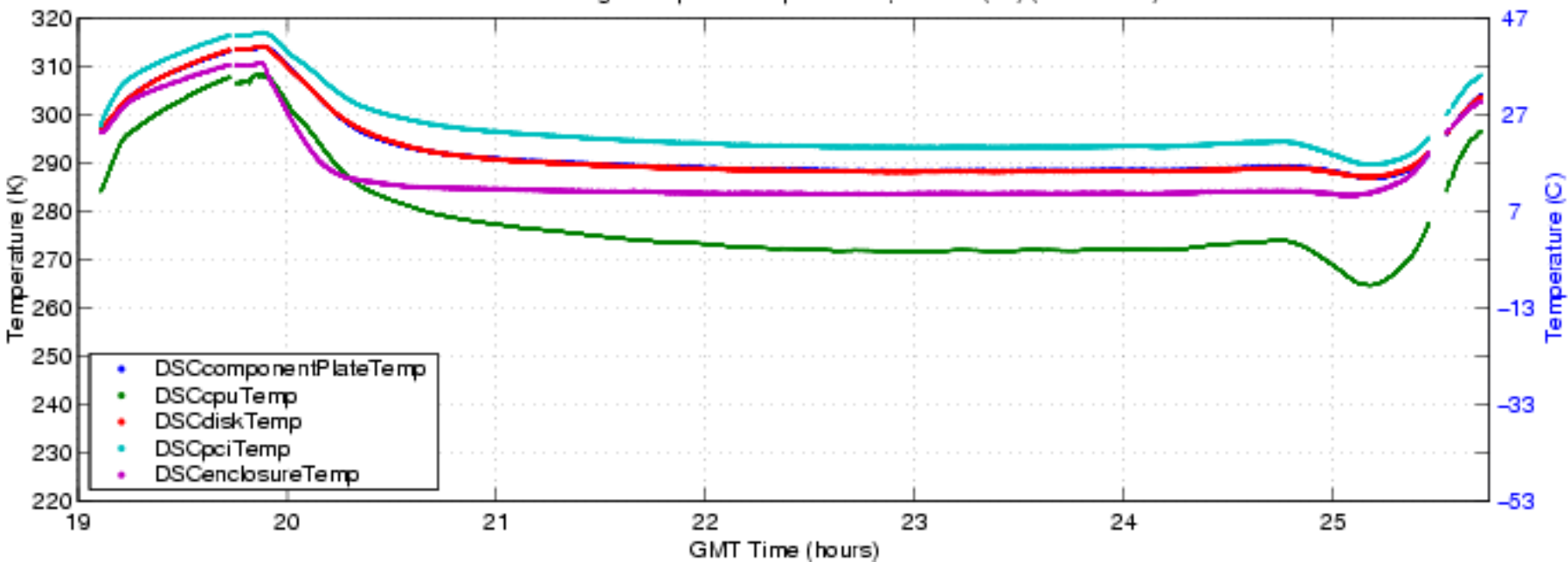
S-HIS Data Storage Computer Temperatures , 041012 (fbf) (ENG Plot 8)
