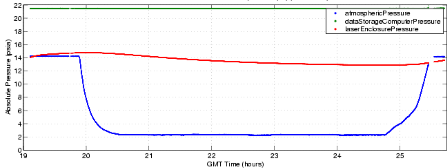
S-HIS Environmental Parameters, 04-10-12 (fbf) (ENG Plot 8)
