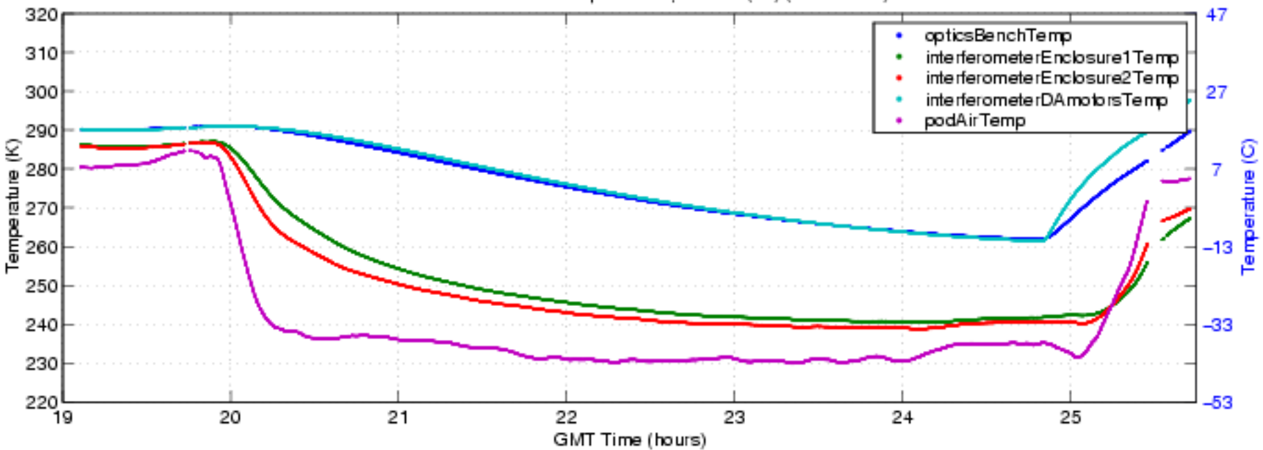
S-HIS Interferometer Temperatures, 041012 (bf) (ENG Plot 5)
