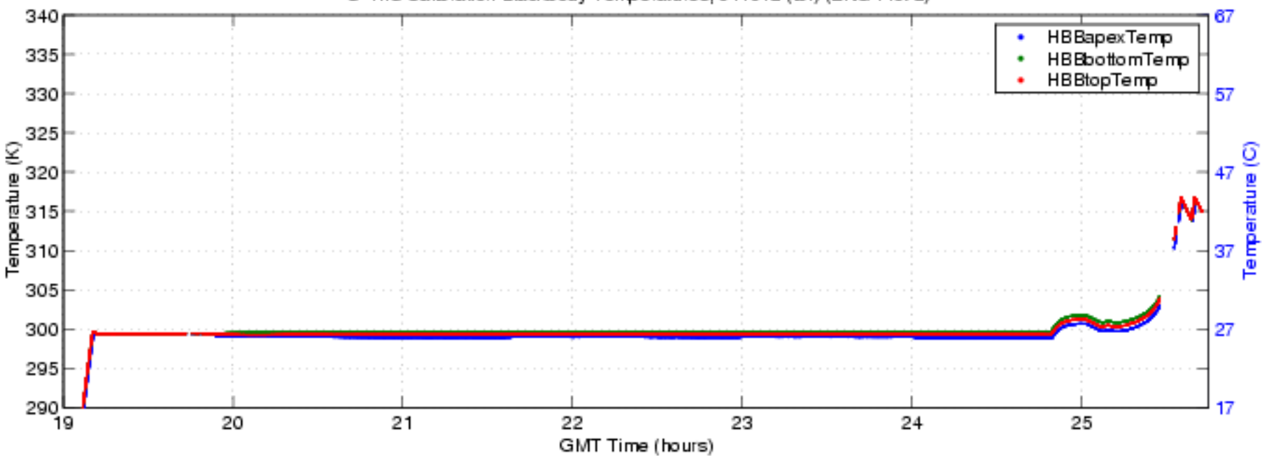
S-HIS Calibration Blackbody Temperatures, 041012 (bf) (ENG Plot 2)
