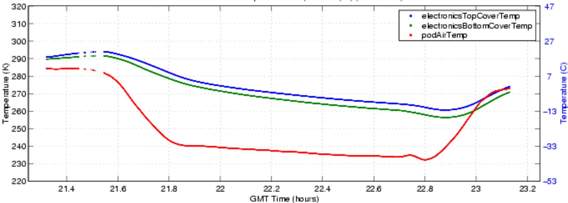
S-HIS Electronics Temperatures 2/2, 04-1010 (fbf) (ENG Plot 8)
