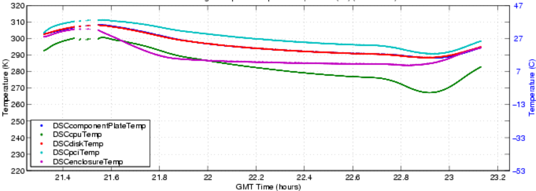
S-HIS Data Storage Computer Temperatures , 041010 (fbf) (ENG Plot 8)
