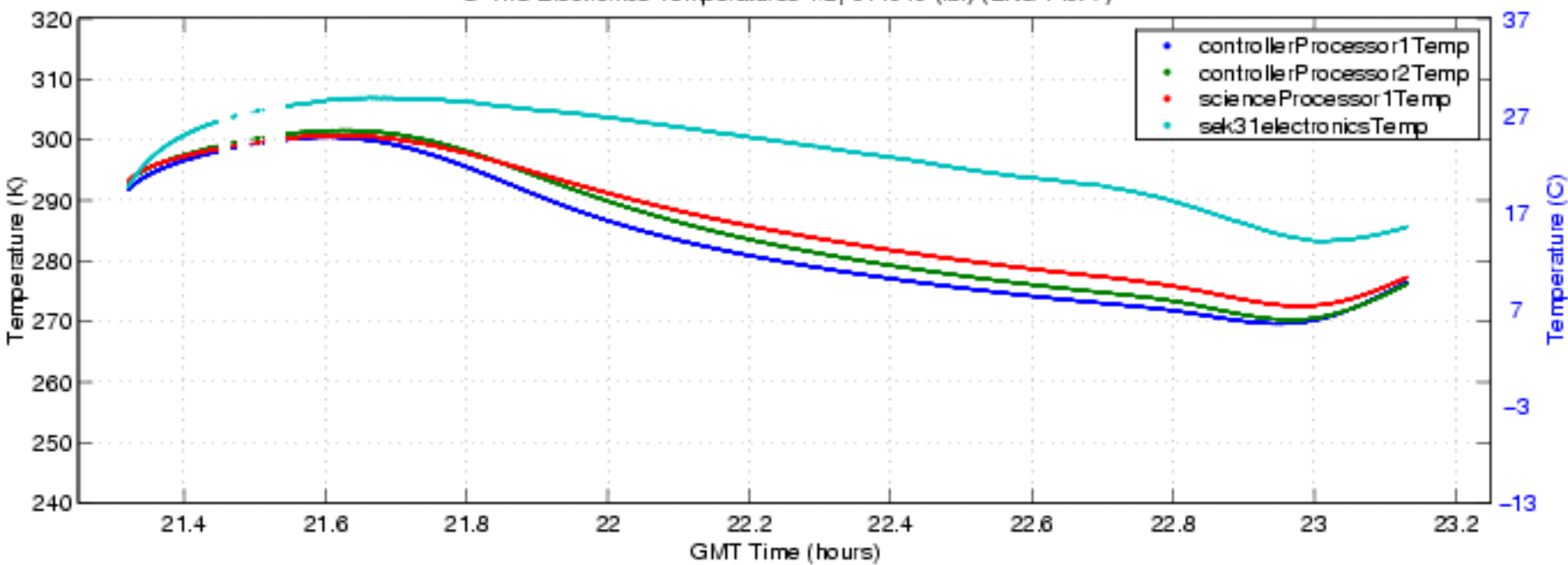
S-HIS Electronics Temperatures 1/2, 04-10-10 (fbf) (ENG Plot 7)
