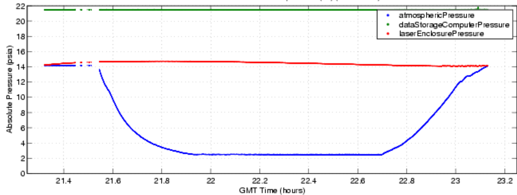
S-HIS Environmental Parameters, 04-10-10 (fbf) (ENG Plot 8)
