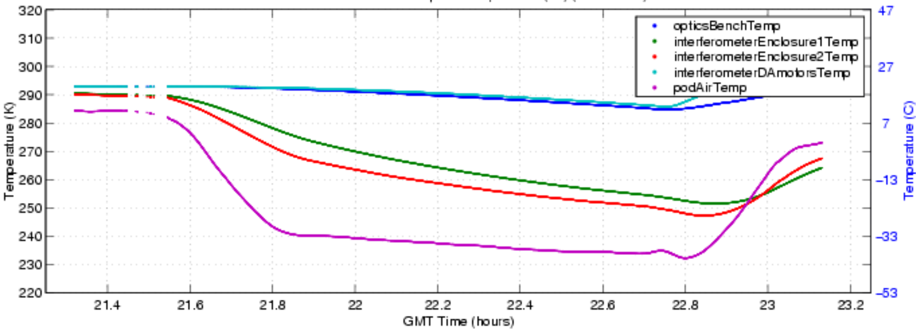
S-HIS Interferometer Temperatures, 041010 (bf) (ENG Plot 5)
