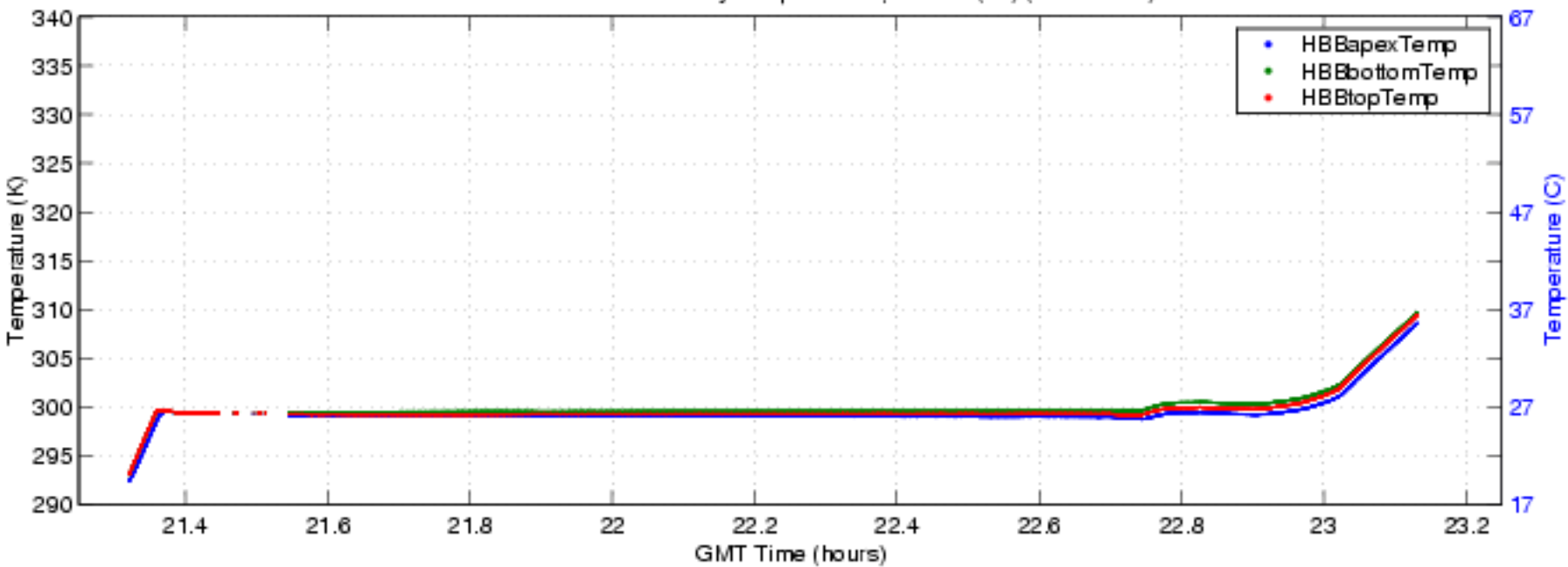
S-HIS Calibration Blackbody Temperatures, 041010 (bf) (ENG Plot 2)
