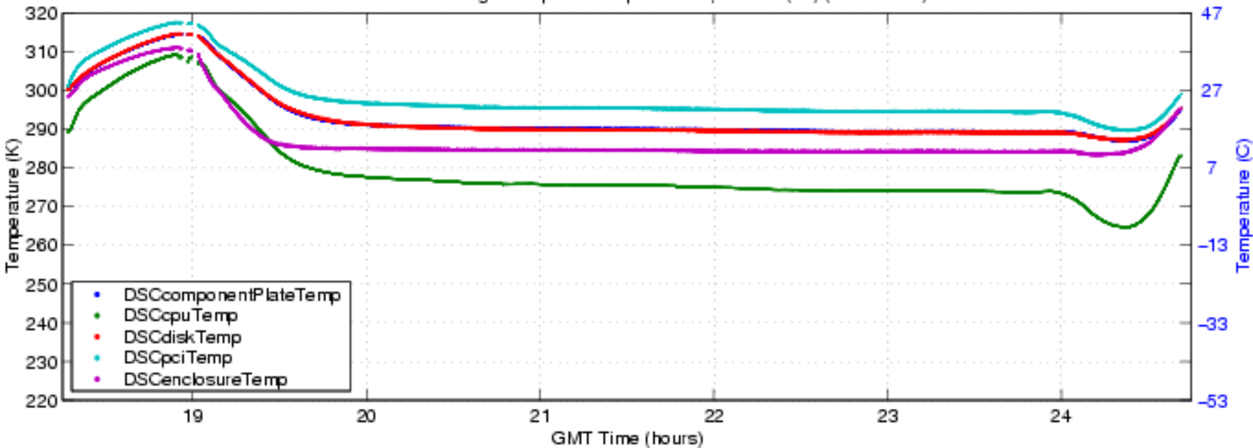
S-HIS Data Storage Computer Temperatures , 041009 (fbf) (ENG Plot 8)
