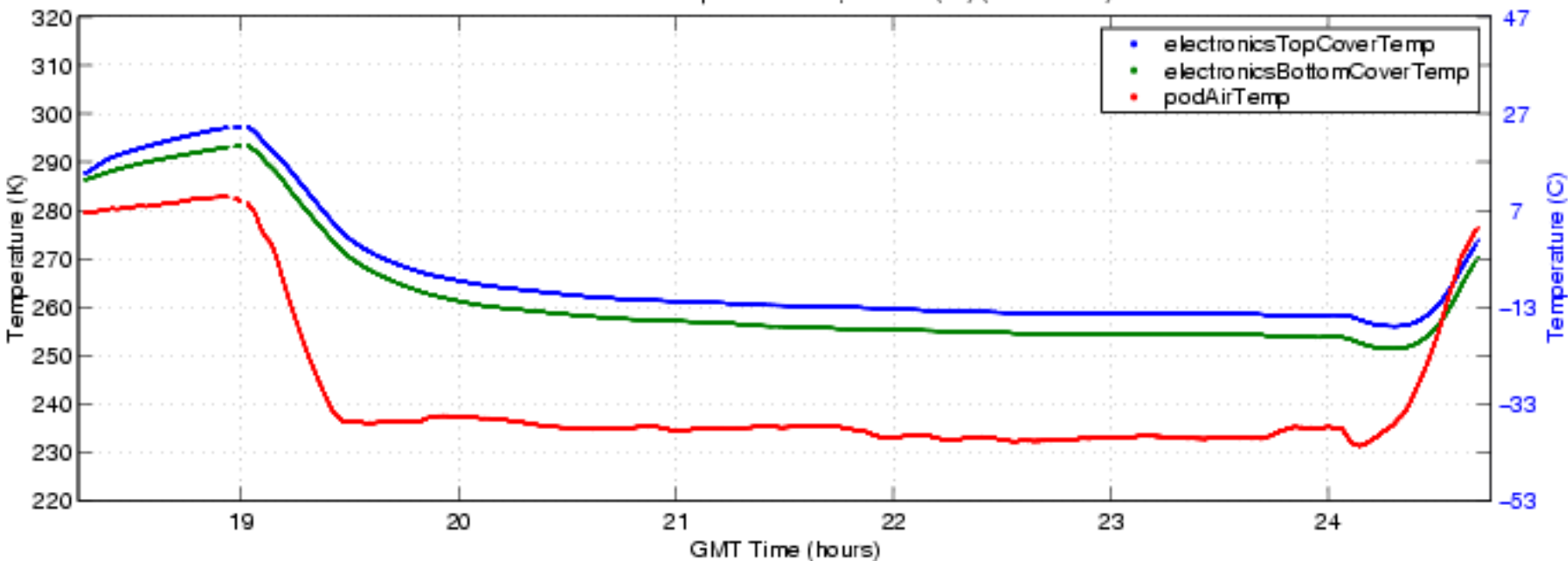
S-HIS Electronics Temperatures 2/2, 04-1009 (fbf) (ENG Plot 8)
