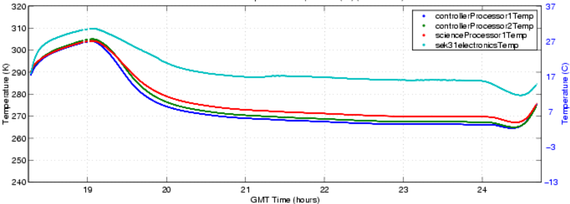
S-HIS Electronics Temperatures 1/2, 04-1009 (fbf) (ENG Plot 7)
