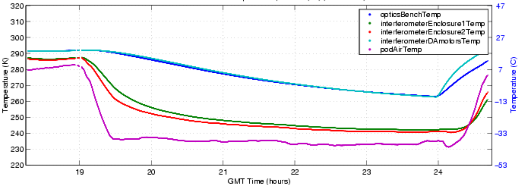
S-HIS Interferometer Temperatures, 041009 (bf) (ENG Plot 5)
