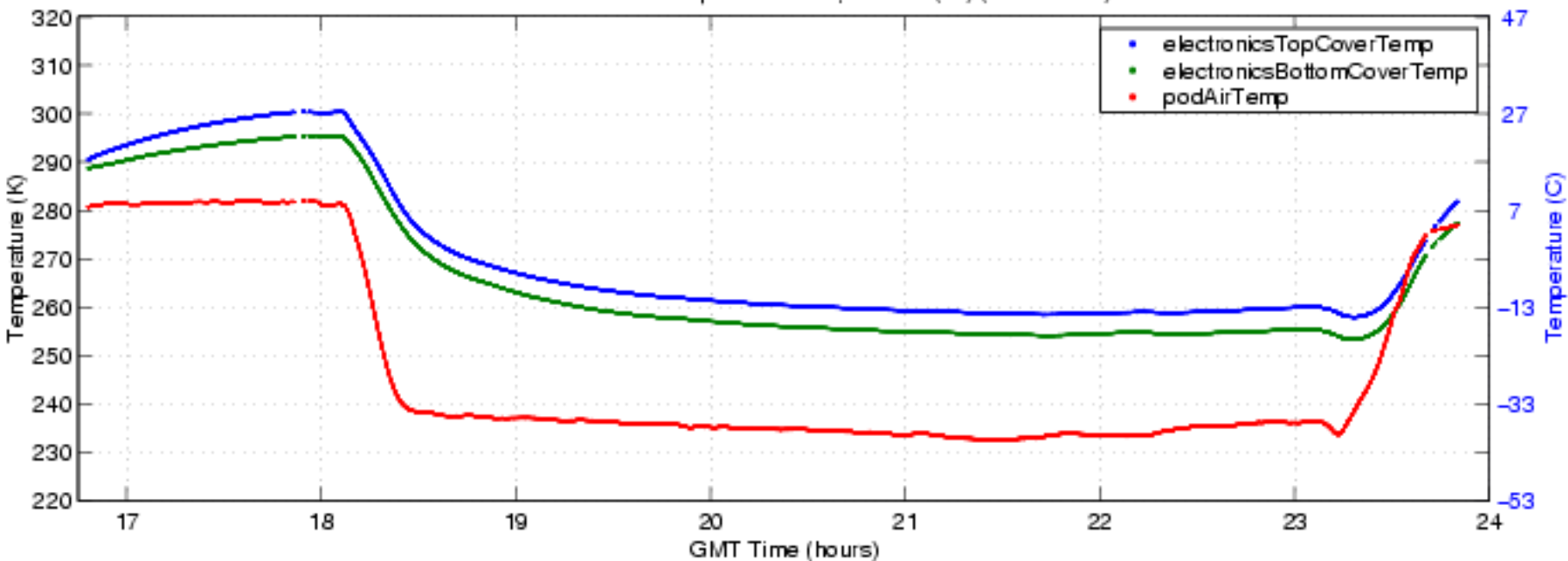
S-HIS Electronics Temperatures 2/2, 04-1008 (fbf) (ENG Plot 8)
