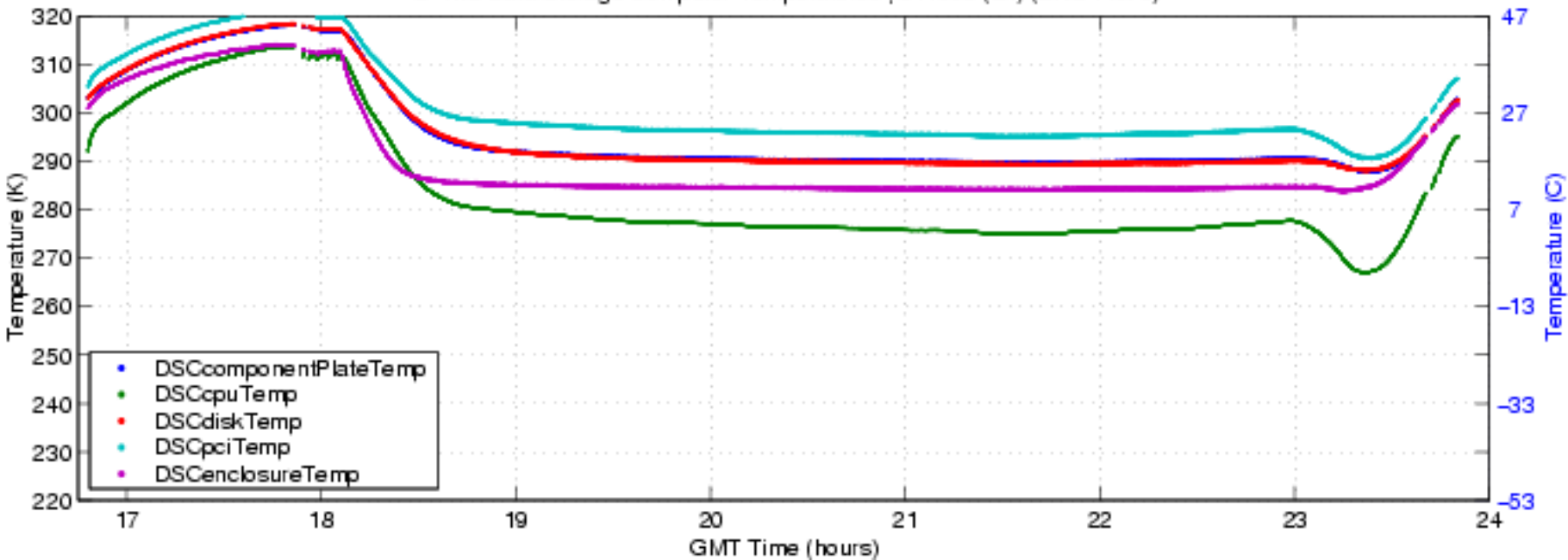
S-HIS Data Storage Computer Temperatures , 041008 (fbf) (ENG Plot 8)
