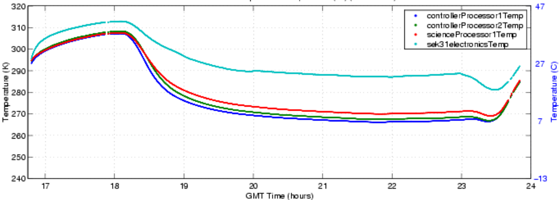
S-HIS Electronics Temperatures 1/2, 04-1008 (fbf) (ENG Plot 7)
