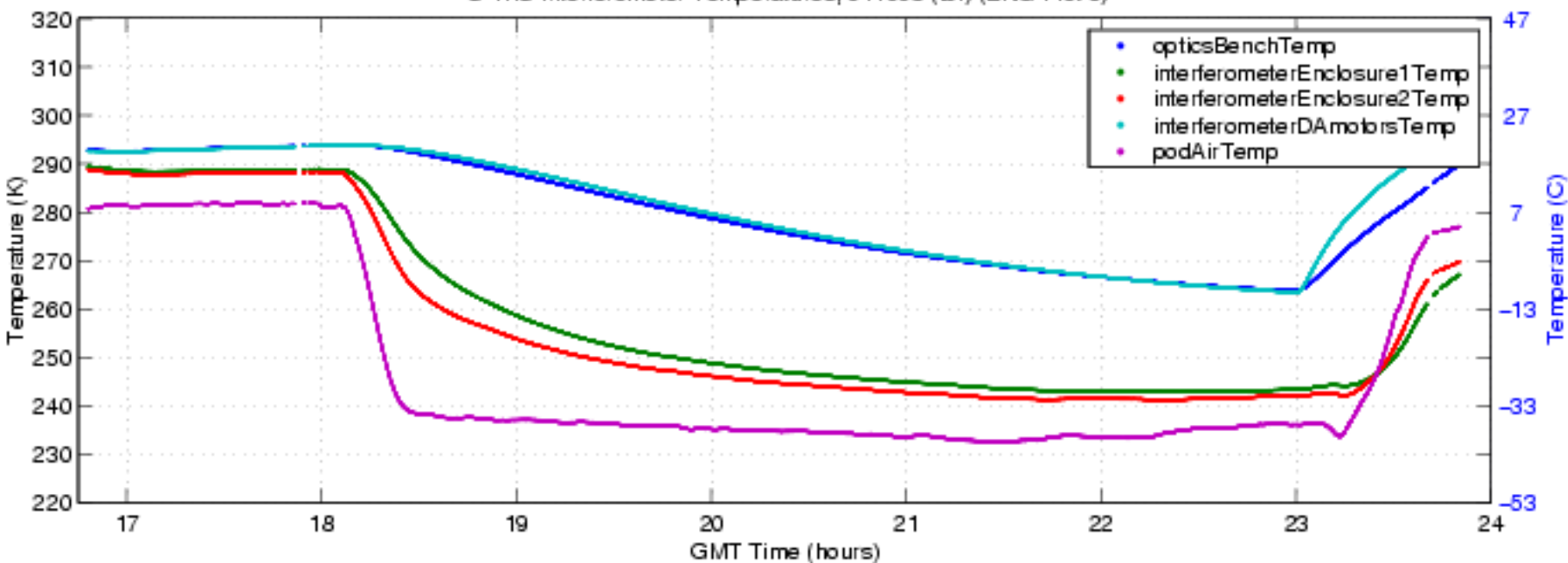
S-HIS Interferometer Temperatures, 041008 (bf) (ENG Plot 5)
