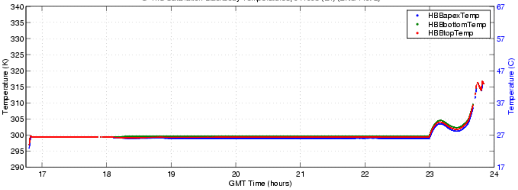
S-HIS Calibration Blackbody Temperatures, 041008 (bf) (ENG Plot 2)
