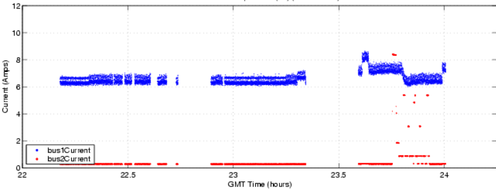
S-HIS Bus Power, 041005 (bf) (ENG Plot 15)
