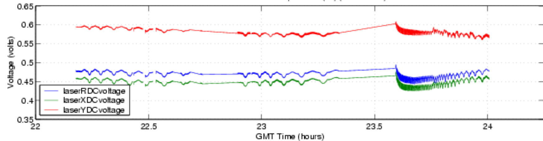
S-HIS Laser Parameters, 041005 (fbf) (ENG Plot 9)
