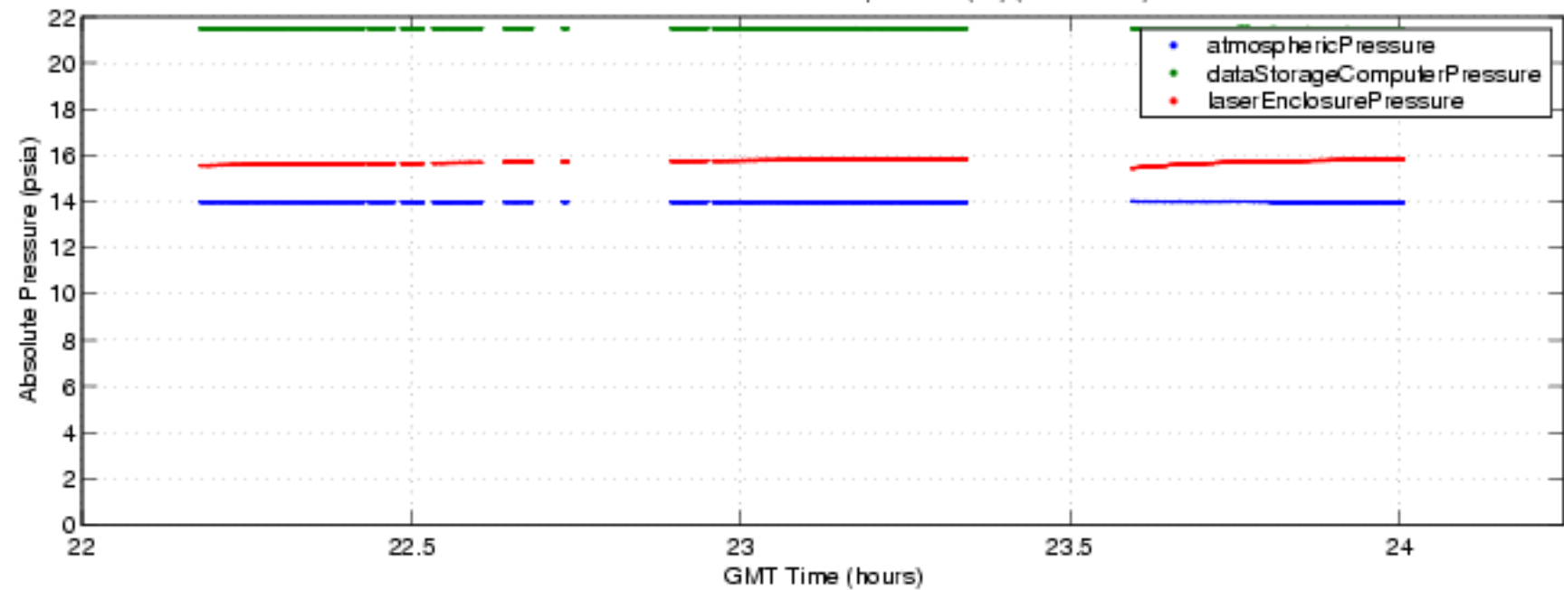
S-HIS Environmental Parameters, 04-1005 (fbf) (ENG Plot 8)
