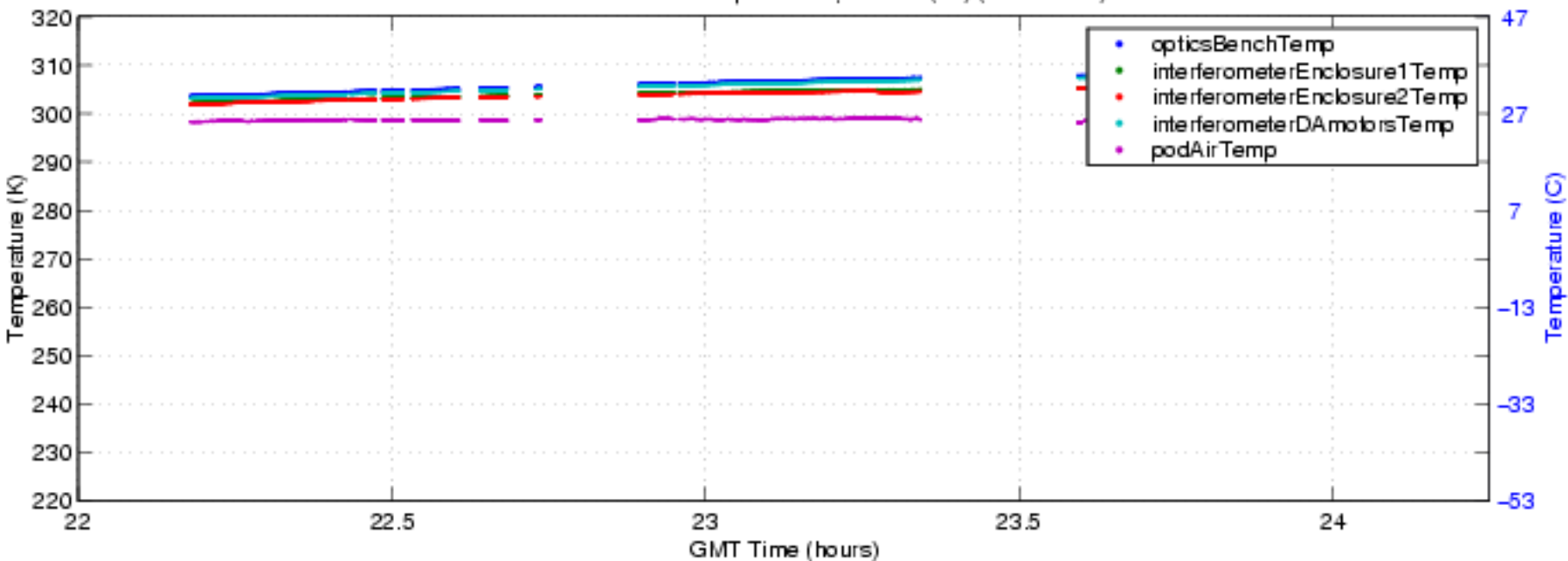
S-HIS Interferometer Temperatures, 041005 (bf) (ENG Plot 5)
