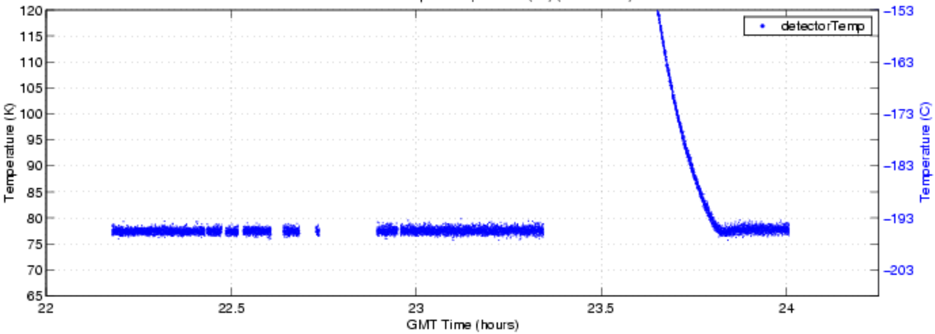
S-HIS Detector Temperature, 041005 (fbf) (ENG Plot 3)
