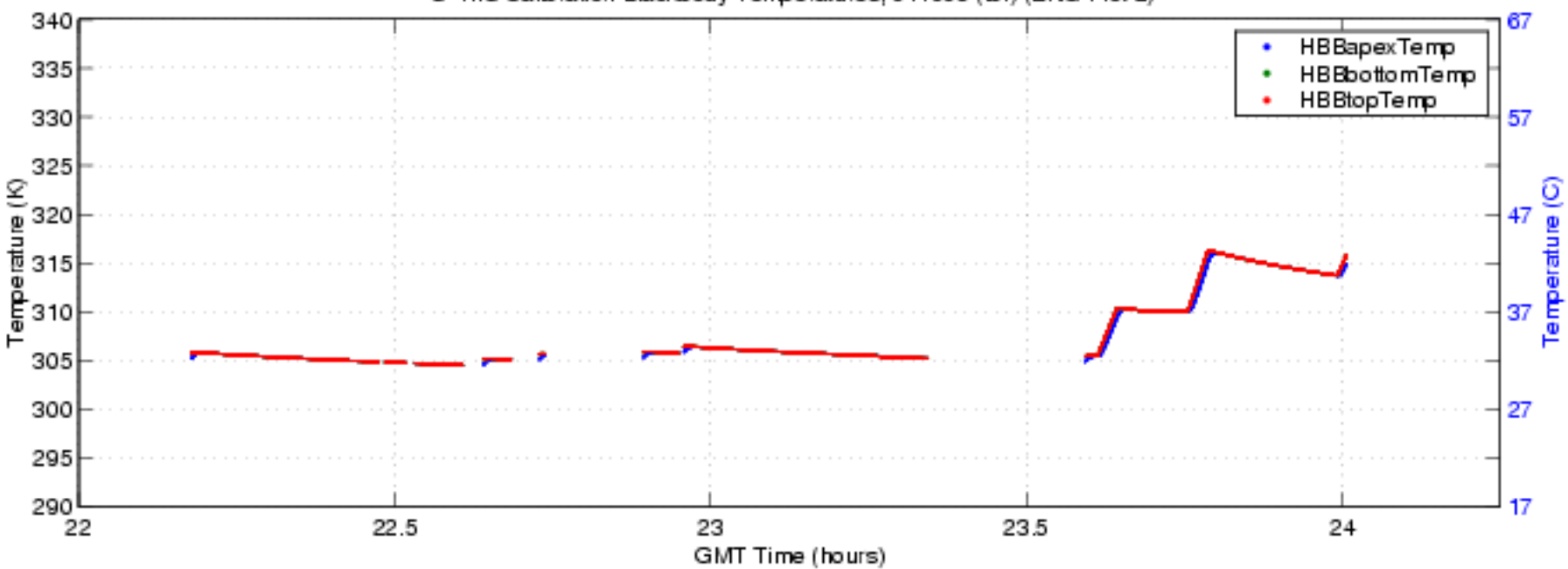
S-HIS Calibration Blackbody Temperatures, 041005 (bf) (ENG Plot 2)
