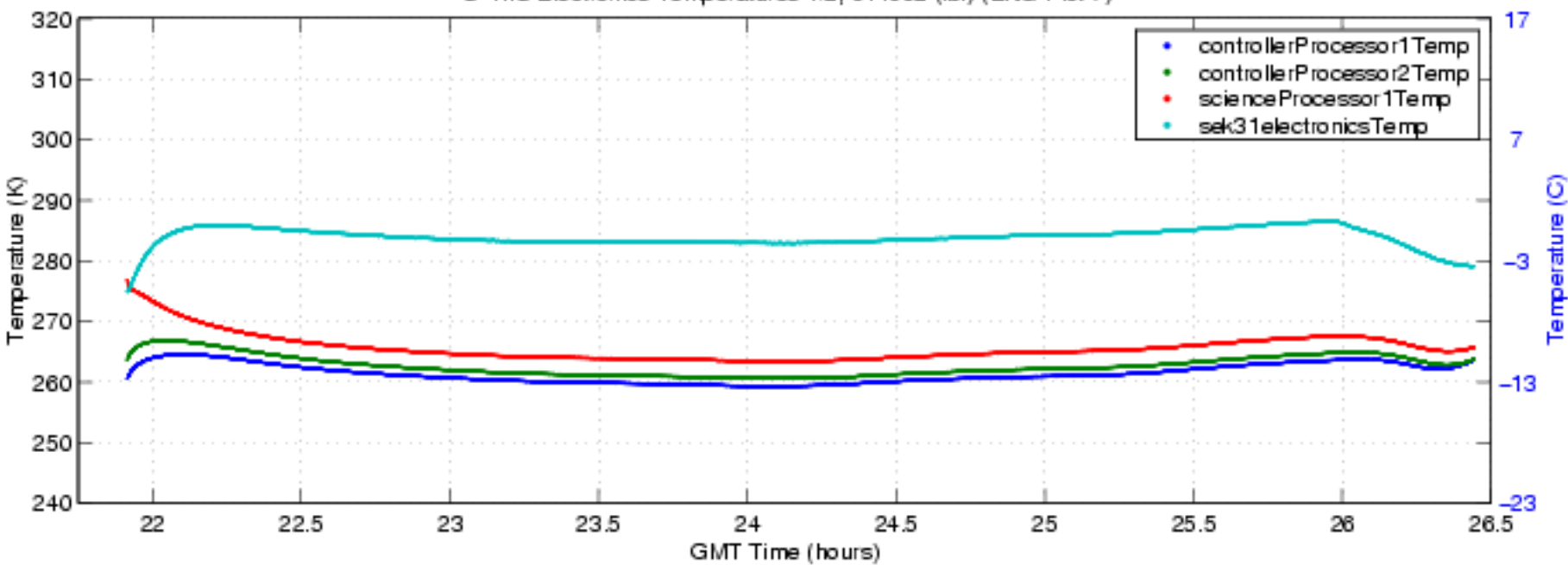
S-HIS Electronics Temperatures 1/2, 04-1002 (fbf) (ENG Plot 7)
