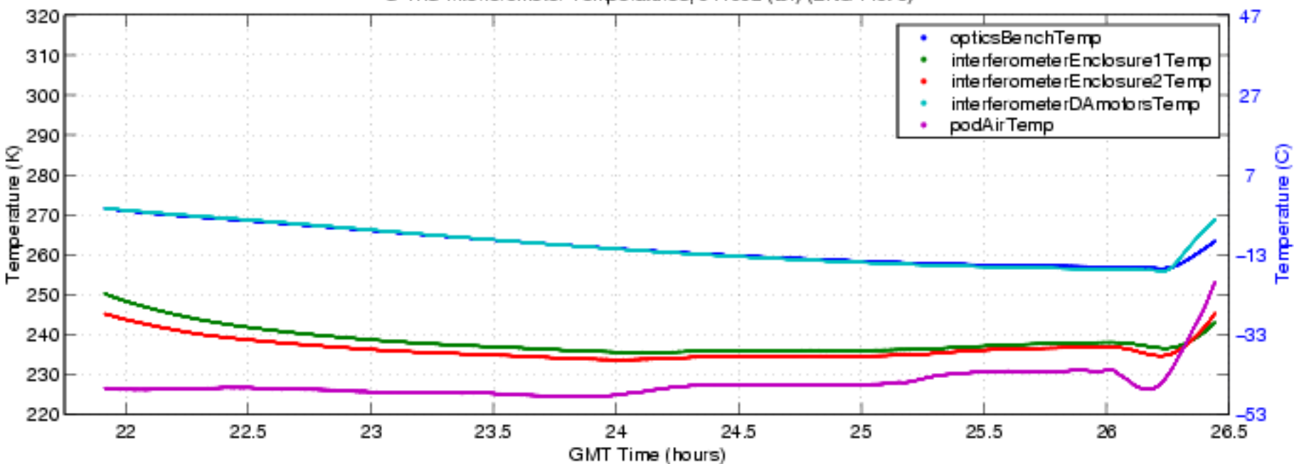
S-HIS Interferometer Temperatures, 041002 (bf) (ENG Plot 5)
