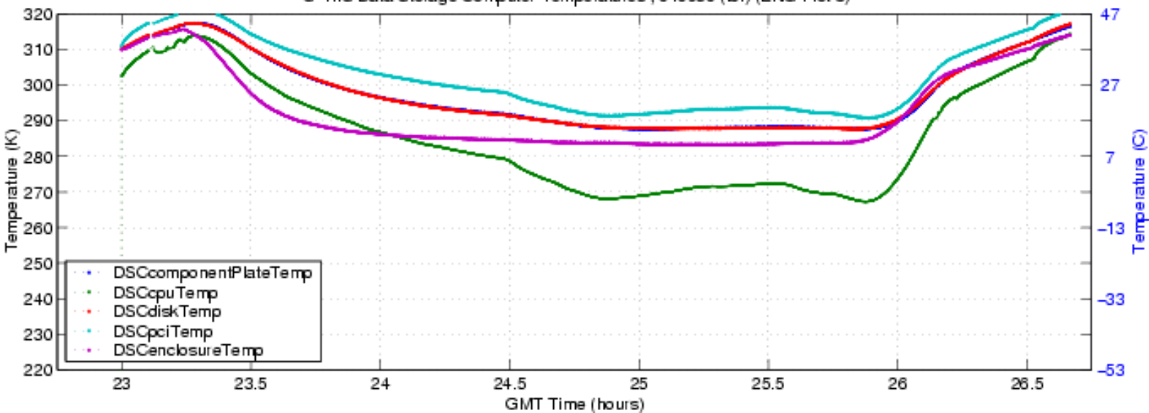
S-HIS Data Storage Computer Temperatures , 040930 (fbf) (ENG Plot 8)
