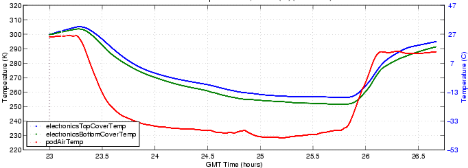
S-HIS Electronics Temperatures 2/2, 040930 (fbf) (ENG Plot 8)
