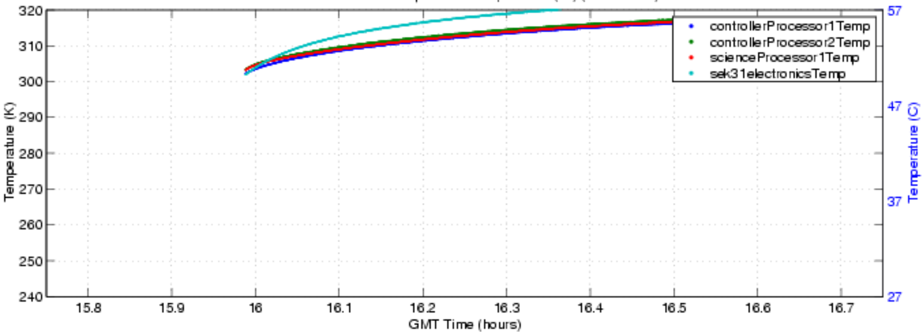
S-HIS Electronics Temperatures 1/2, 041023 (fbf) (ENG Plot 7)
