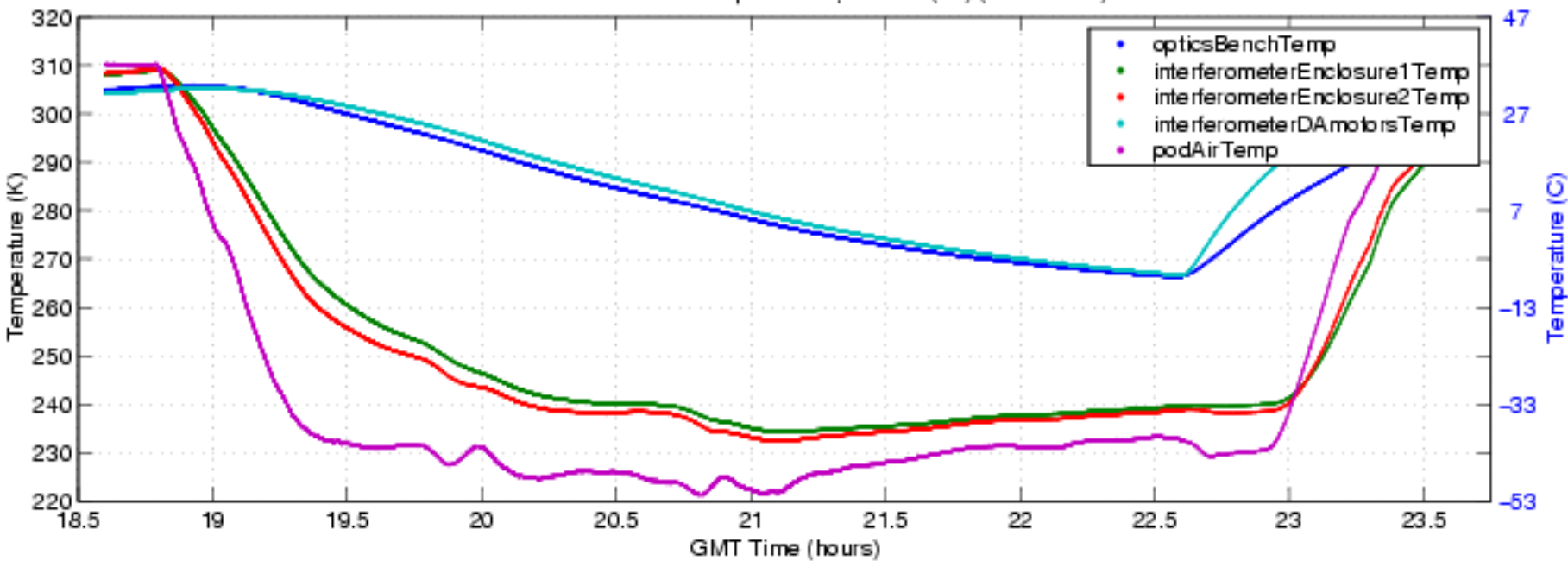
S-HIS Interferometer Temperatures, 050619 (bf) (ENG Plot 6)
