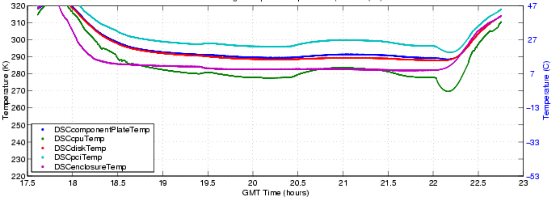
S-HIS Data Storage Computer Temperatures , 050615 (fbf)
