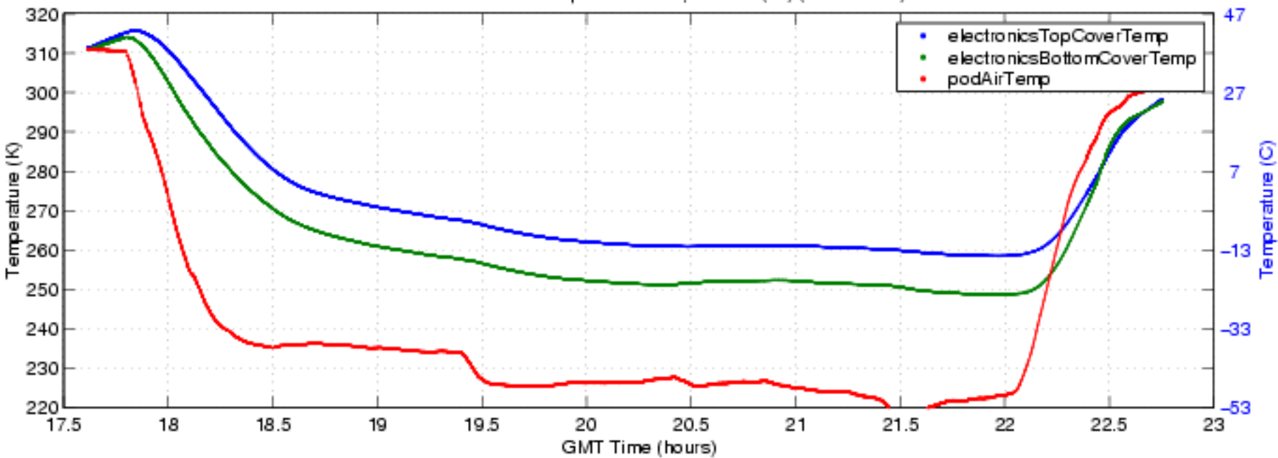
S-HIS Electronics Temperatures 2/2, 050615 (fbf) (ENG Plot 9)
