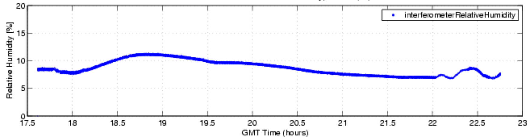
S-HIS Interferometer Relative Humidity, 050615 (fbf)
