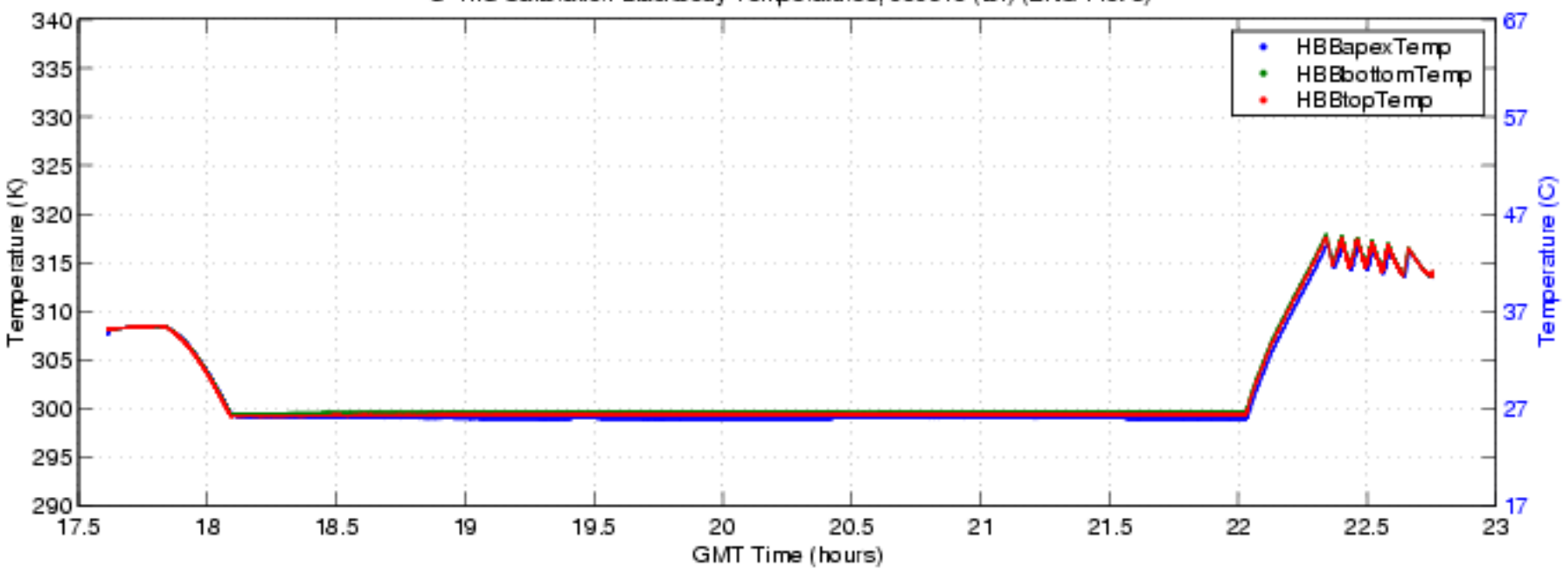
S-HIS Calibration Blackbody Temperatures, 050615 (bf) (ENG Plot 3)
