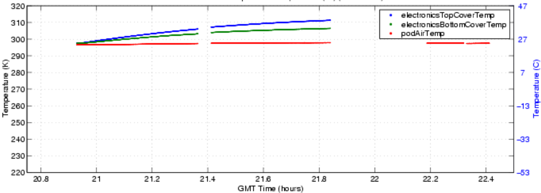
S-HIS Electronics Temperatures 2/2, 050614 (fbf) (ENG Plot 9)
