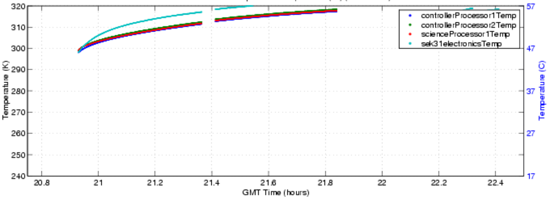
S-HIS Electronics Temperatures 1/2, 050814 (fbf) (ENG Plot 8)
