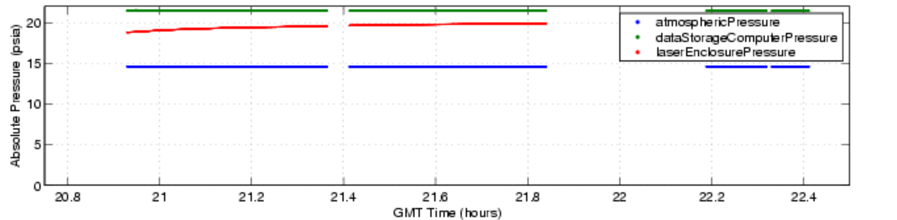
S-HIS Environmental Parameters, 050614 (fbf) (ENG Plot 7)
