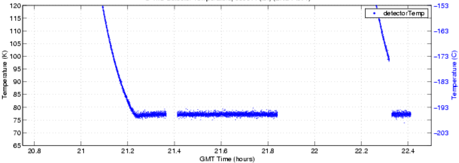
S-HIS Detector Temperature, 050614 (fbf) (ENG Plot 4)
