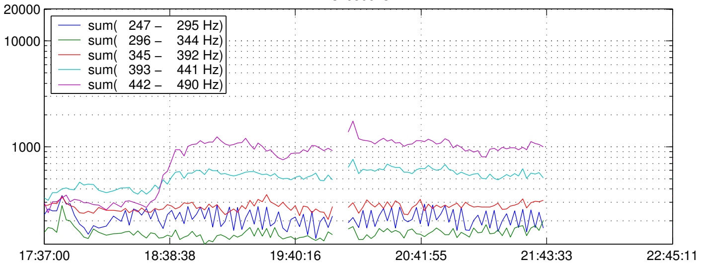
Tilt Power (binned by frequency) vs Time sh050613
