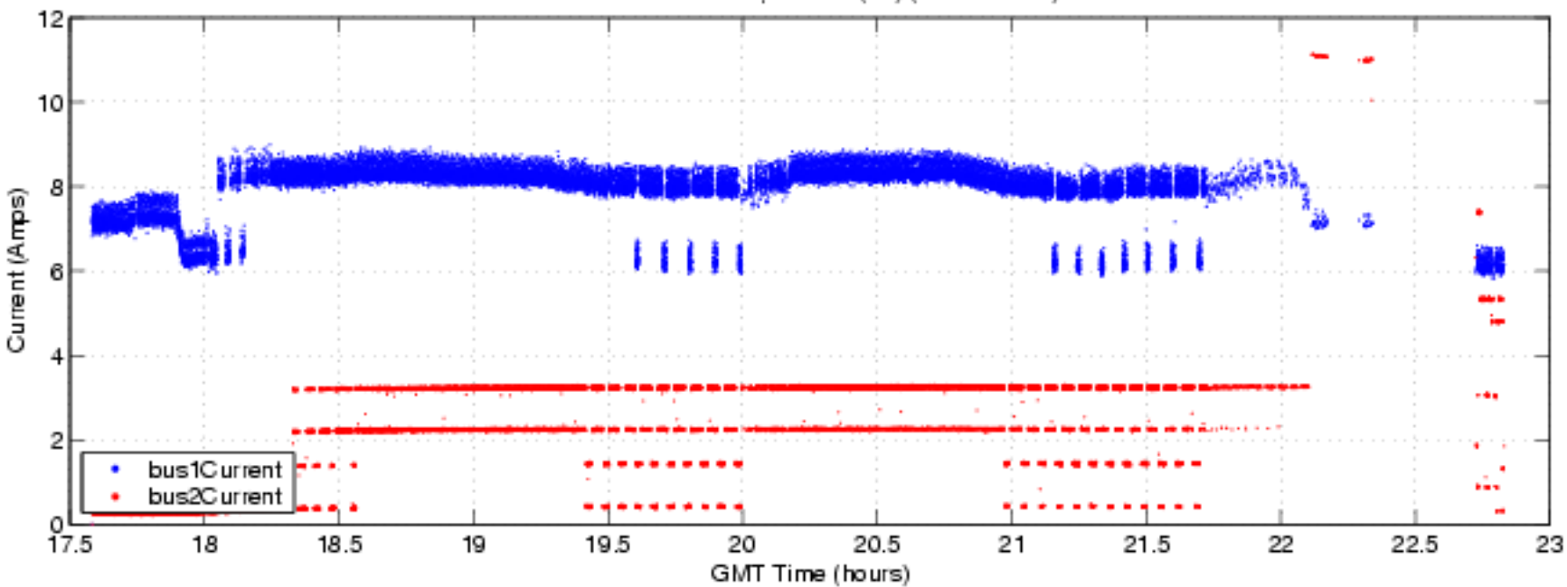
S-HIS Bus Power, 050613 (bf) (ENG Plot 16)
