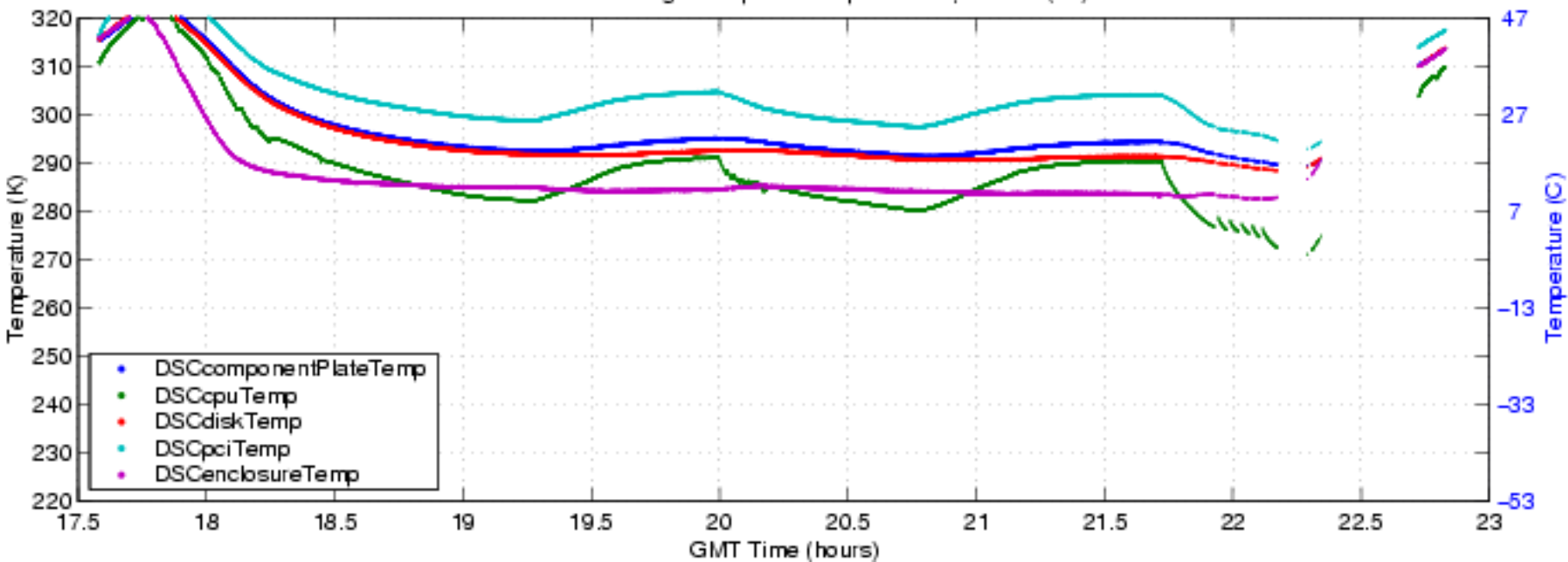
S-HIS Data Storage Computer Temperatures , 050613 (fbf)
