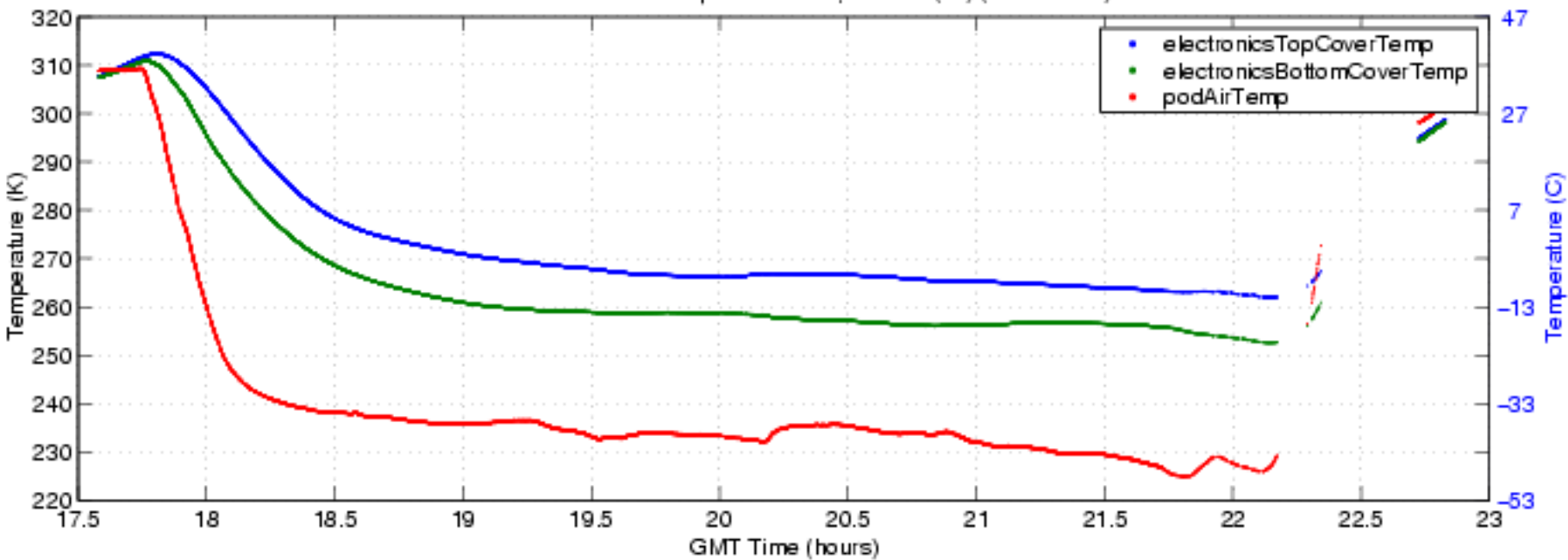
S-HIS Electronics Temperatures 2/2, 050613 (fbf) (ENG Plot 9)
