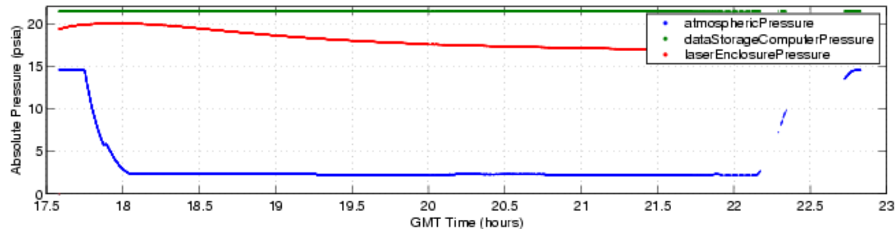
S-HIS Environmental Parameters, 050613 (fbf) (ENG Plot 7)
