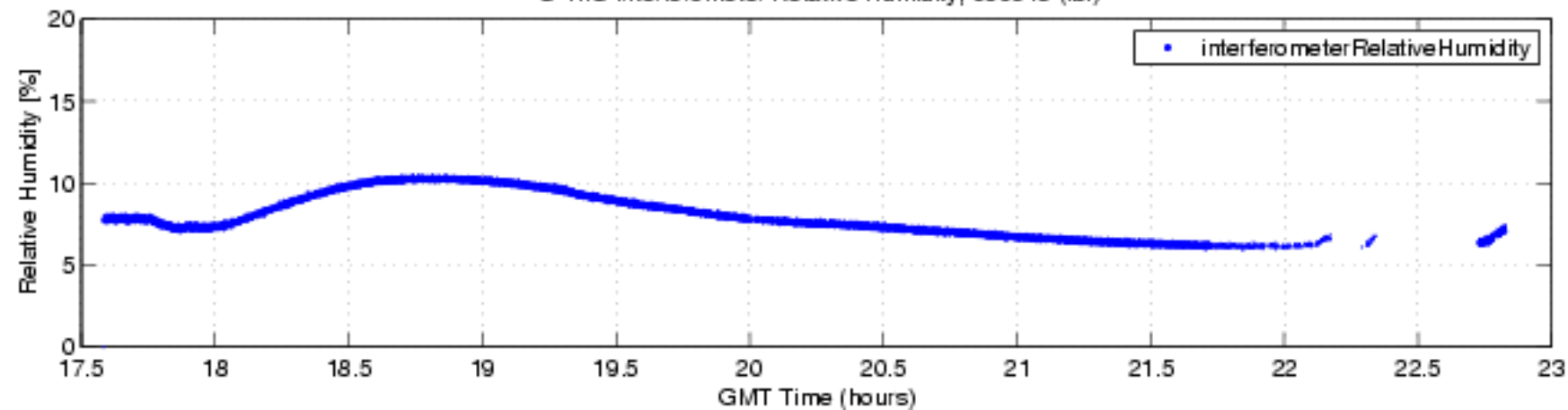
S-HIS Interferometer Relative Humidity, 050613 (fbf)
