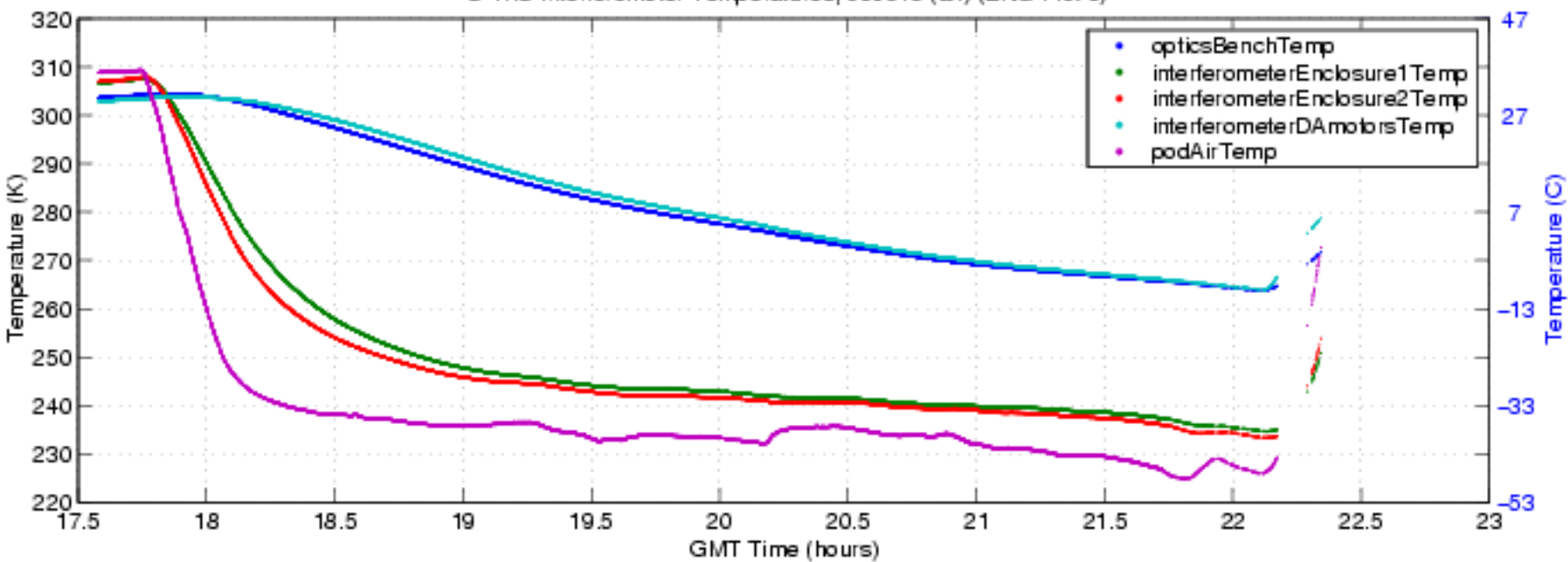
S-HIS Interferometer Temperatures, 050613 (bf) (ENG Plot 6)
