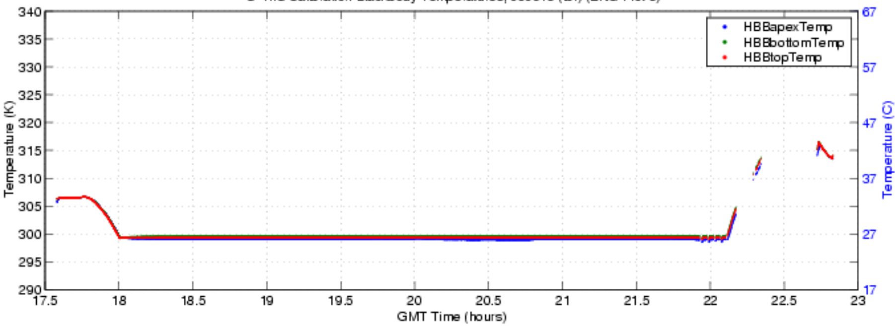
S-HIS Calibration Blackbody Temperatures, 050613 (bf) (ENG Plot 3)
