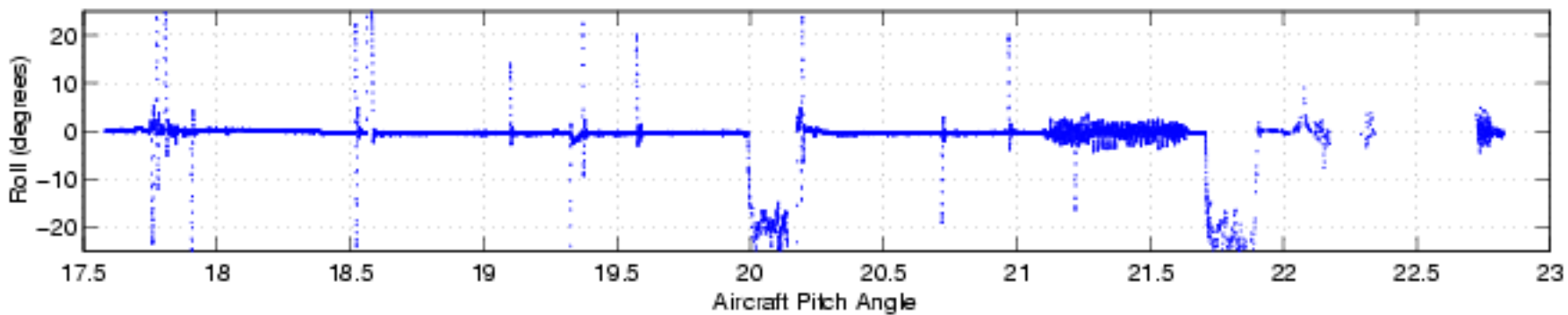
Aircraft Roll Angle 050813 (fbf) (ENG Plot 2)
