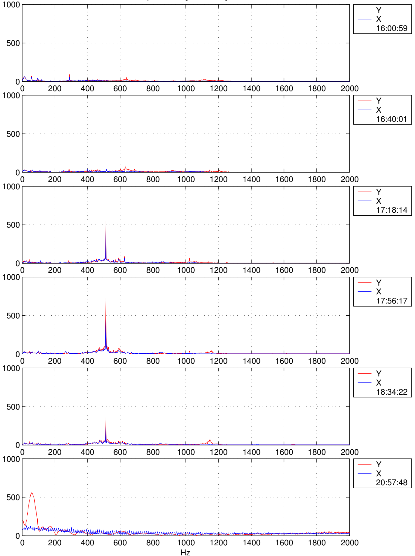
DA Tilt Error Angle Power Spectrum Number of samples averaged: 10; flight date: 050611
