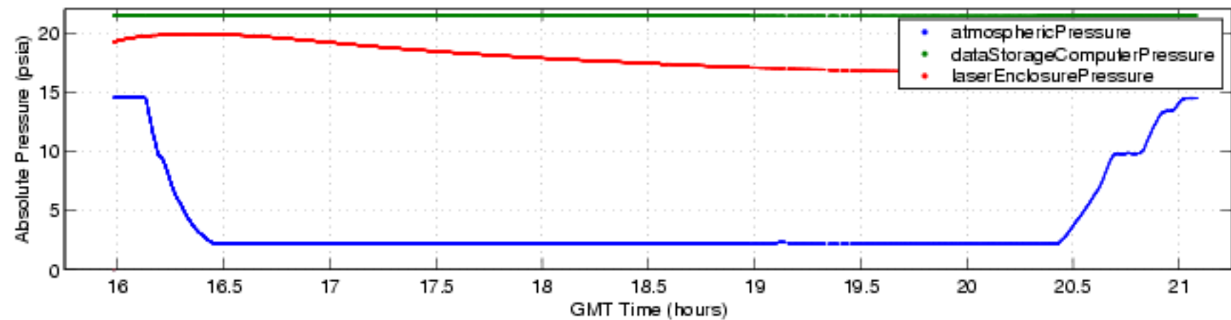
S-HIS Environmental Parameters, 050611 (fbf) (ENG Plot 7)
