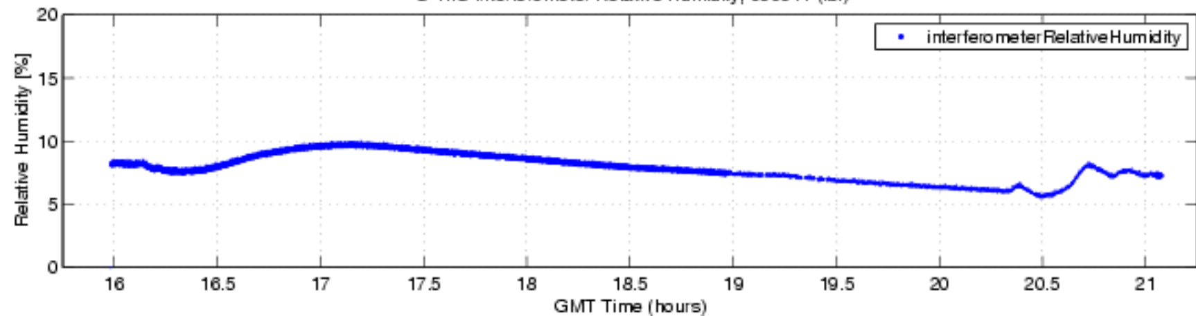
S-HIS Interferometer Relative Humidity, 050611 (fbf)
