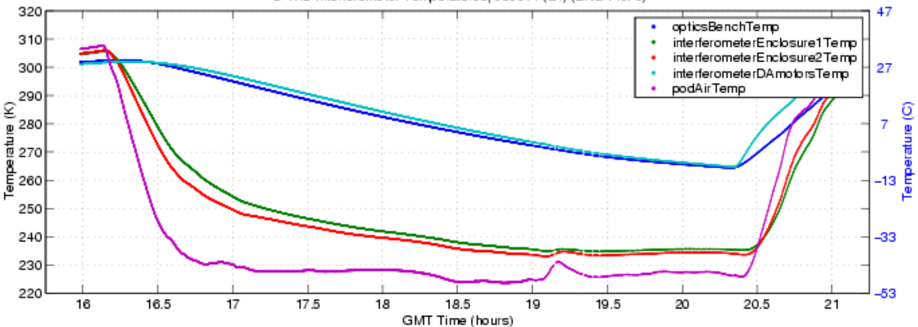
S-HIS Interferometer Temperatures, 050611 (bf) (ENG Plot 6)
