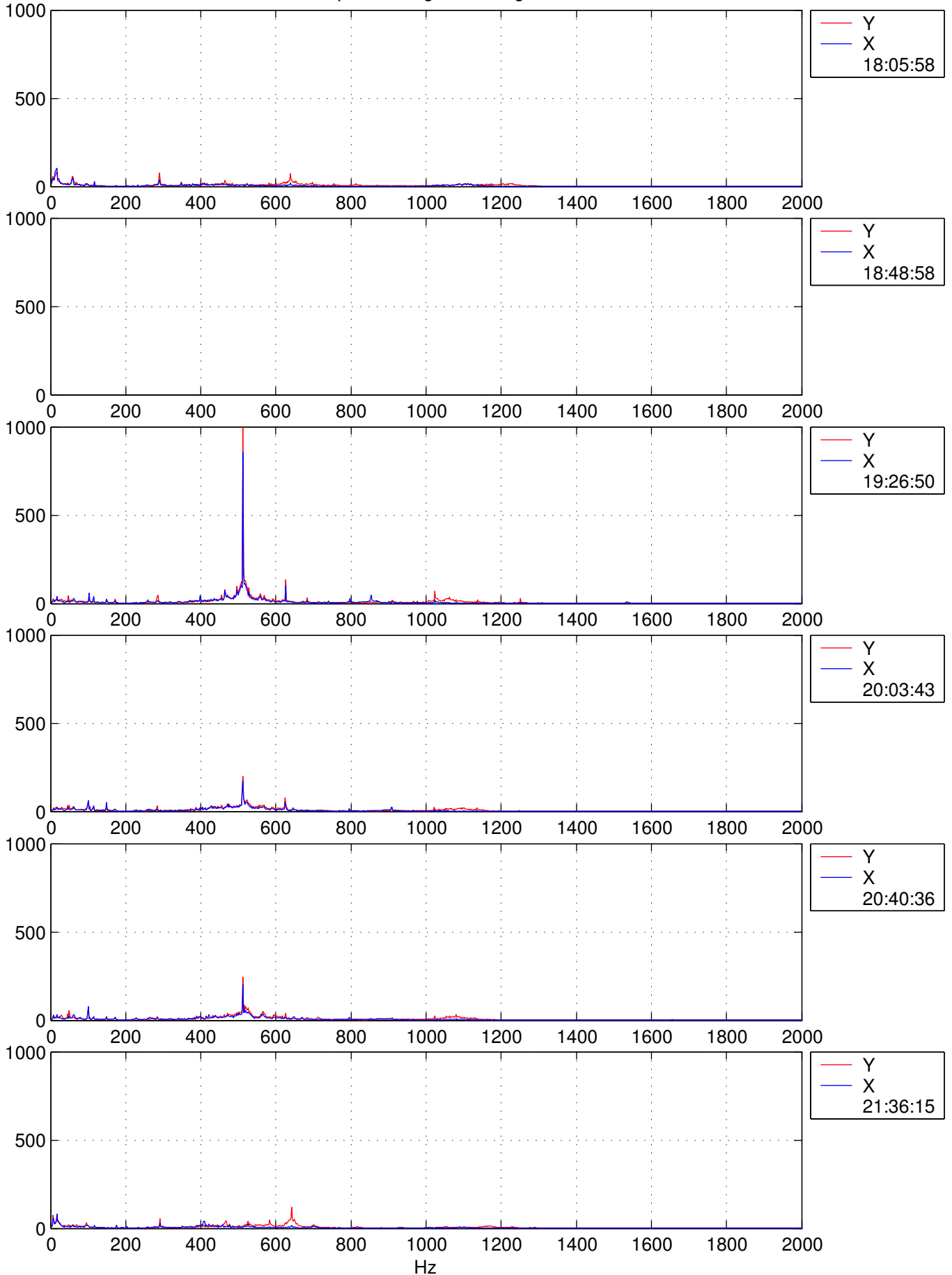
DA Tilt Error Angle Power Spectrum Number of samples averaged: 10; flight date: 050609
