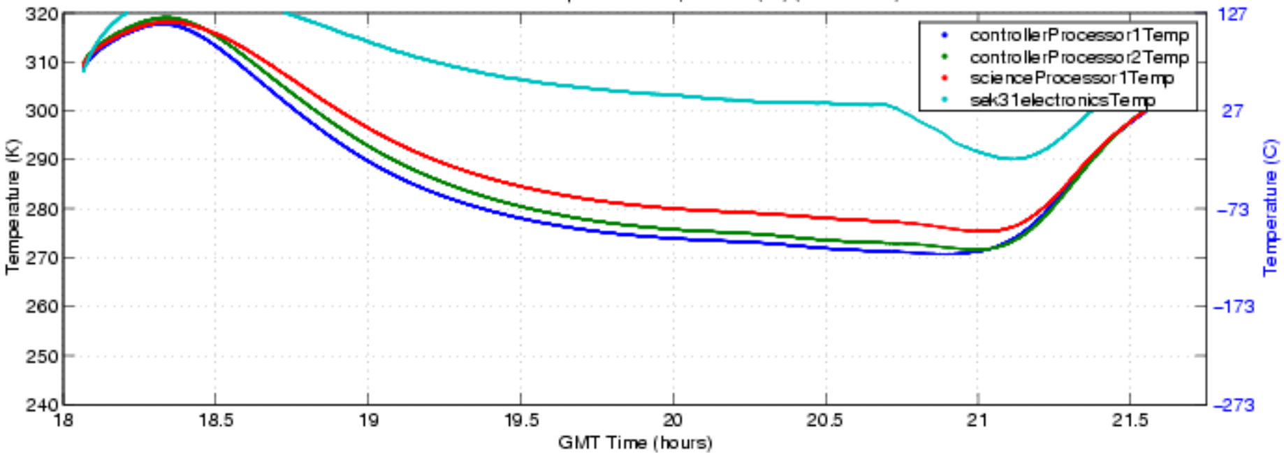
S-HIS Electronics Temperatures 1/2, 050809 (fbf) (ENG Plot 8)
