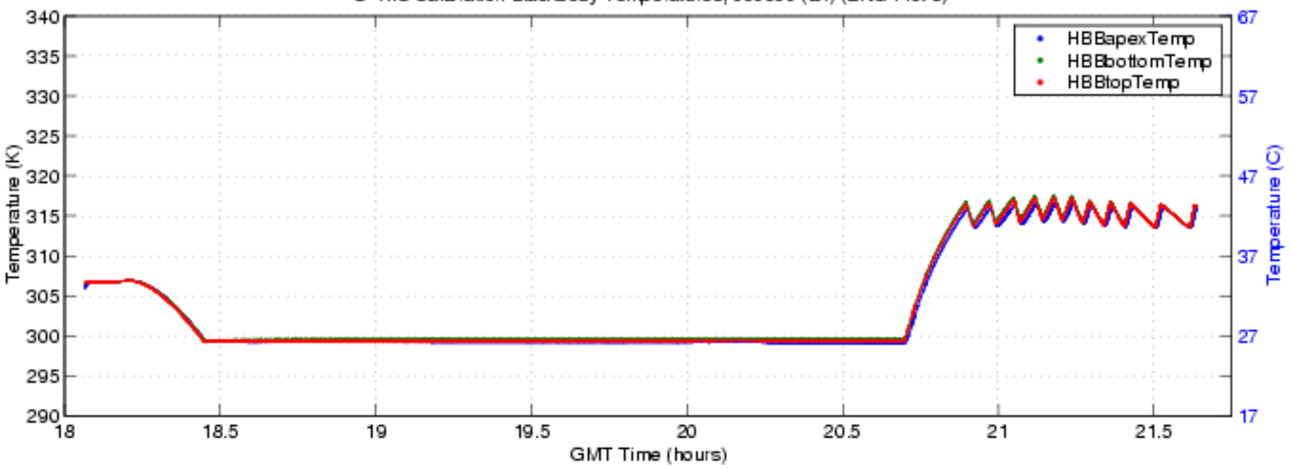
S-HIS Calibration Blackbody Temperatures, 050609 (bf) (ENG Plot 3)
